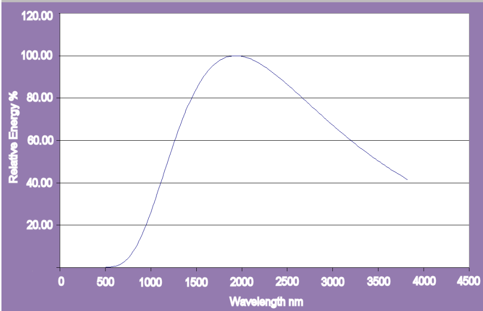
Relative Energy Spectral Curve of a 220v/1200w NDA Lamp
